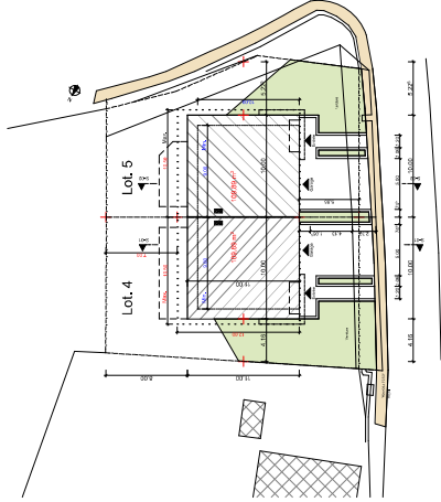
Implantation 1:250
